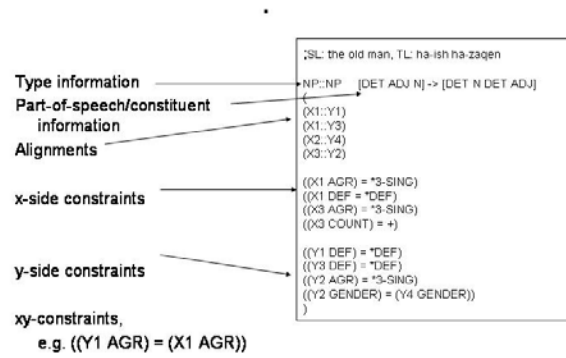
Figure 3. An Example Transfer Rule along with its Components
