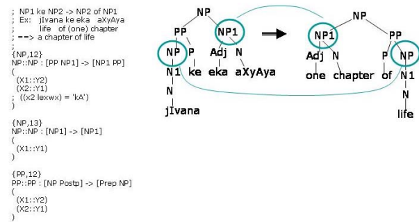
Figure 4. Recursive NP and PP Transfer Rules for Hindi to English Translation
