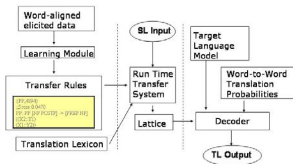
Figure 1. Architecture of the XFER MT System and its Major Components
