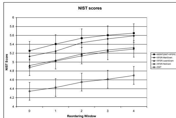
Figure 5. Results by NIST Score with Various Reordering Windows.
