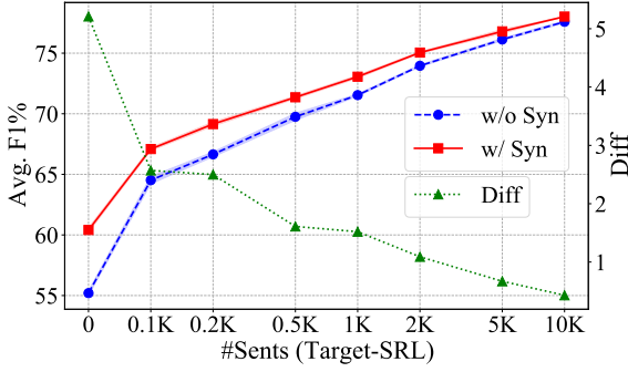
Figure 6: Averaged UPB development results versus number of SRL target sentences (in log scale) utilized per target language (using XLM-R for encoder).
