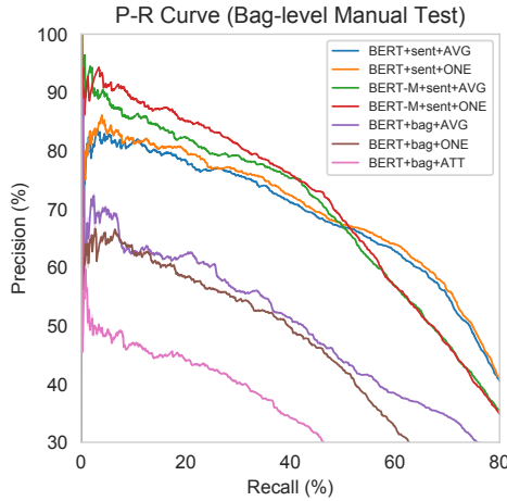
Figure 4: Comparisons of different DS-RE models with BERT on NYT10 bag-level manual test set.
