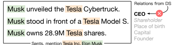
Figure 1: Typical errors made by DS evaluation. In the figure, DS labels the bag with only the relation CEO, while none of the sentences express the relation. Also, it misses a correct relation shareholder due to the incompleteness of the knowledge graphs.
