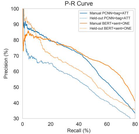
Figure 3: Comparisons of using bag-level manual test (solid lines) and corresponding held-out test (dotted lines). Both absolute and relative scores of models significantly change when taking on human-labeled data.
