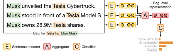
Figure 2: An illustration for a typical multi-instance multi-label (bag-level) model. The model aims to predict relation probabilities for entity pairs, instead of sentences, which is usually accomplished by aggregating a bag representation and doing classification over it.
