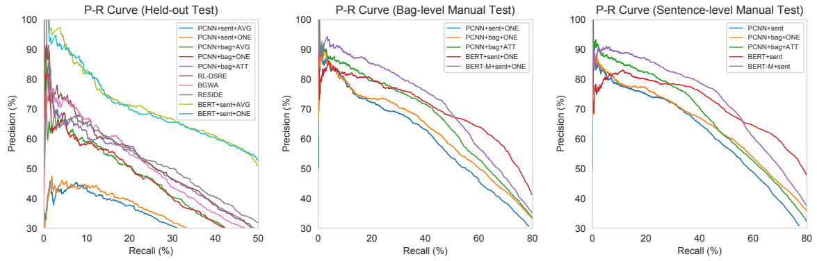
Figure B.1: P-R curves of representative models in held-out test, bag-level manual test and sentence-level manual test of NYT10. Note that the scales of X-axis are not the same in the three figures.
