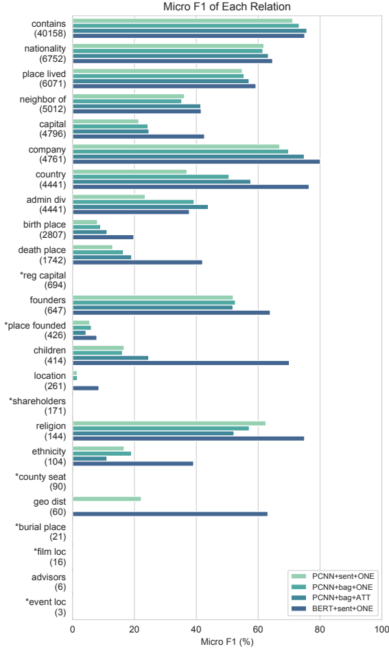
Figure 5: Micro F1 (%) of different relations on the bag-level manual test of NYT10. * represents the relation has less than 20 sentences in the test sets. Numbers in brackets are numbers of training sentences.
