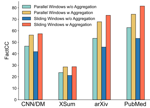
Figure 3: The factual consistency of sliding generation with aggregation and without aggregation.
